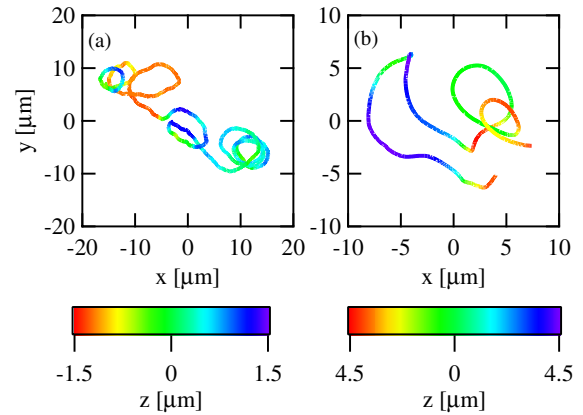
Figure 1. Example trajectories of 3D bead motion. Data are shown for a bead moving in the 2 \mu\text{m} (a) and 80 \mu\text{m} (b) chambers. The color scale denotes the z -position, the position along the microscope optical axis.
