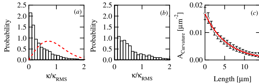
Figure 3. (a) The 3D curvature probability distribution. The probability of measured curvatures for all beads using the 80\ \mu\text{m} chambers is displayed (bars, n = 15 ). The curvature has been normalized by its RMS value from each run. For comparison, the distribution predicted by Rutenberg and Grant [21] is shown (red dotted line). (b) The normalized curvature distribution for all runs using the 2\ \mu\text{m} chambers is displayed ( n = 13 ). (c) Autocorrelation of the path curvature. The autocorrelation of the curvature as a function of path length for a single bead trajectory (open circles) and a fit of this data to a single exponential decay (red solid line).
