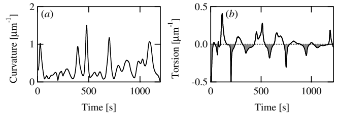
Figure 2. The calculated curvature (a) and torsion (b) as a function of time for the example trajectory shown in figure 1(b) from a bead moving in an 80 \mu\text{m} chamber. (b) Open shading denotes times during which the trajectory torsion is positive and thus moving with a right-handed component. Gray shading denotes left-handed sections. Note that the torsion crosses zero multiple times and thus the bead trajectory is not predominantly right or left handed.
