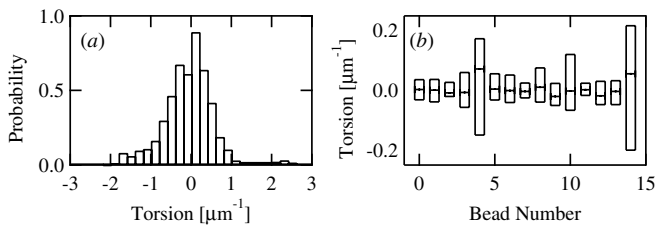
Figure 4. (a) The torsion probability distribution. The torsion of measured curvatures for all beads using the 80\ \mu\text{m} chambers is displayed ( n = 15 ). (b) Box plot of the curvature distribution from each of the 15 individual beads whose data is compiled in (a). The three horizontal lines represent the 25th, 50th, and 75th percentiles of each set of torsions.
