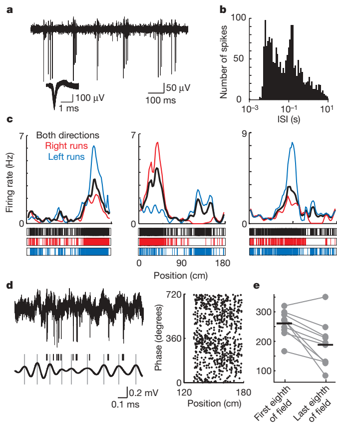
Figure 3 | Extracellular recordings of CA1 place cells along the virtual linear track. a , An example extracellular recording filtered between 500 Hz and 7.5 kHz. The inset shows overlaid spike waveforms from the recording. b , ISI distribution for the full duration of the recording shown in a . The time axis is plotted on a log scale. c , Example firing rate maps for 3 place cells from 3 different mice. Top, firing rates at positions along the track are shown for rightward runs (red), leftward runs (blue) and runs in either direction (black). Bottom, the position on the track of each spike in the recording is shown as a vertical line. A total of 23 place cells from 8 mice were recorded. d , Phase precession of spike times relative to LFP theta. Top left, an example extracellular recording, filtered between 2 Hz and 10 kHz, during a run through the place field. Spikes and the LFP were recorded on the same electrode. Bottom left, the extracellular recording band-pass filtered between 6 and 10 Hz. Grey lines denote peaks ( 0^\circ ) in the filtered trace, black lines denote the times of spikes. Right, an example plot of phase (two cycles) versus position on the virtual track for all spikes during complete runs through the place field for a single cell. e , Phase values for spikes in the first and last eighth of the place field. Connected points represent a single place field. Horizontal lines indicate the means. n = 10 place fields from 8 cells and 3 mice (multiple place fields are owing to the directionality of firing rates).
