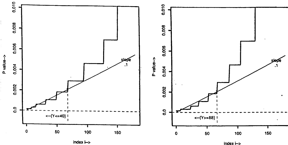
Figure 3: Application of FDR-controlling algorithm to BRCA1/BRCA2 comparison, \alpha = .10 , p_o = 1.0 . Left Panel: Step function shows ordered p-values for one-sided Wilcoxon tests that reject for small values of rank sum statistic Y_i ; \mathcal{R}_{.10} procedure (3.4) rejects for the 68 genes having Y_i \leq 40 . Right Panel: Same, rejecting for large values of Y_i ; \mathcal{R}_{.10} rejects for the 66 genes with Y_i \geq 88 .
