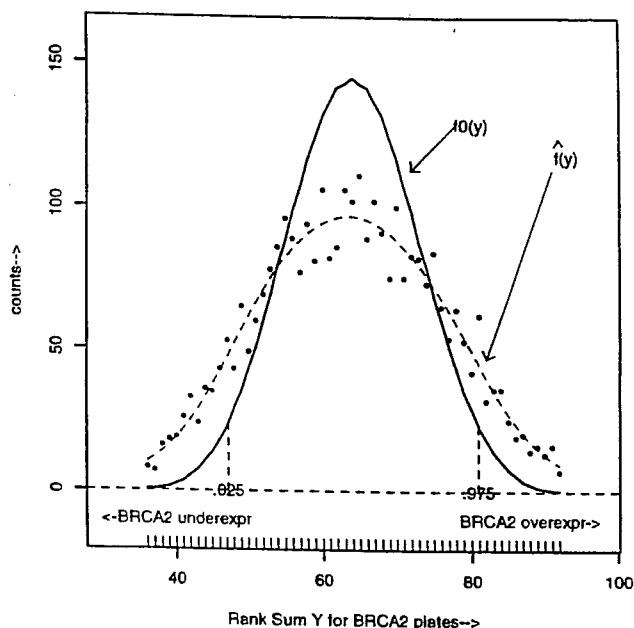
Figure 1: Rank sum statistics comparing BRCA1 vs BRCA2 for the 3226 genes; points are actual counts, solid curve show expected counts under the null hypothesis of no activity differences. Dashed curve is a Poisson regression fit to the actual counts, as explained in Section 2.
