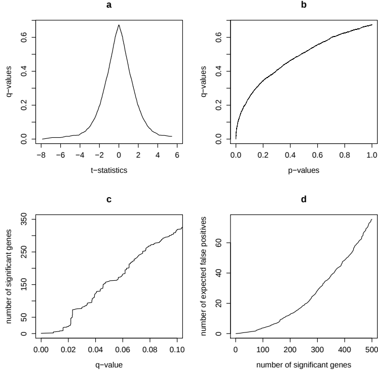
Figure 2: Results from the Hedenfalk et al. data. (a) The q -values of the genes versus their respective t -statistics. (b) The q -values versus their respective p -values. (c) The number of genes occurring on the list up through each q -value versus the respective q -value. (d) The expected number of false positive genes versus the total number of significant genes given by the q -values.
