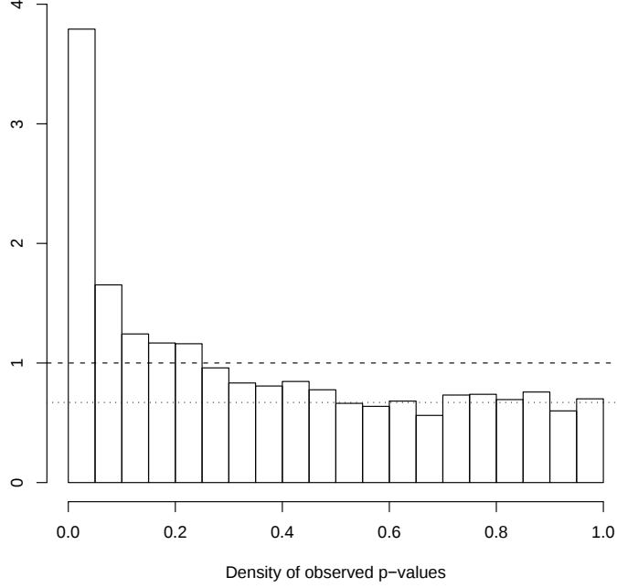
Figure 1: A density histogram of the 3170 p -values from the Hedenfalk et al. data. The dashed line is the density histogram we would expect if all genes were null (not differentially expressed). The dotted line is at the height of our estimate of the proportion of null p -values.
